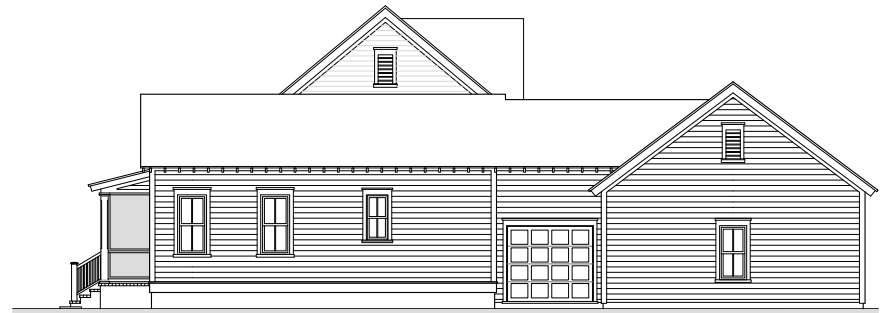
LEFT ELEVATION
